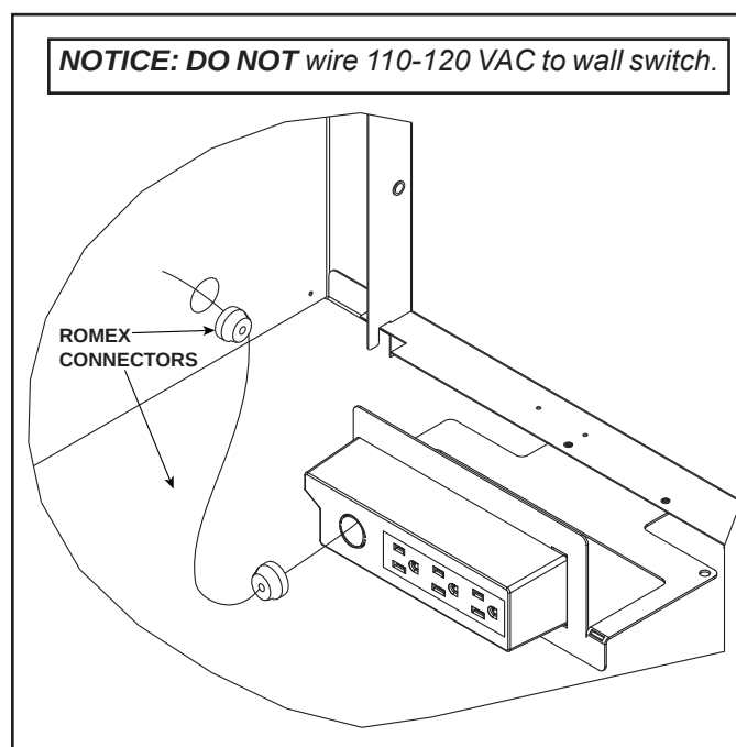
Figure 8.1 Junction Box Detail
