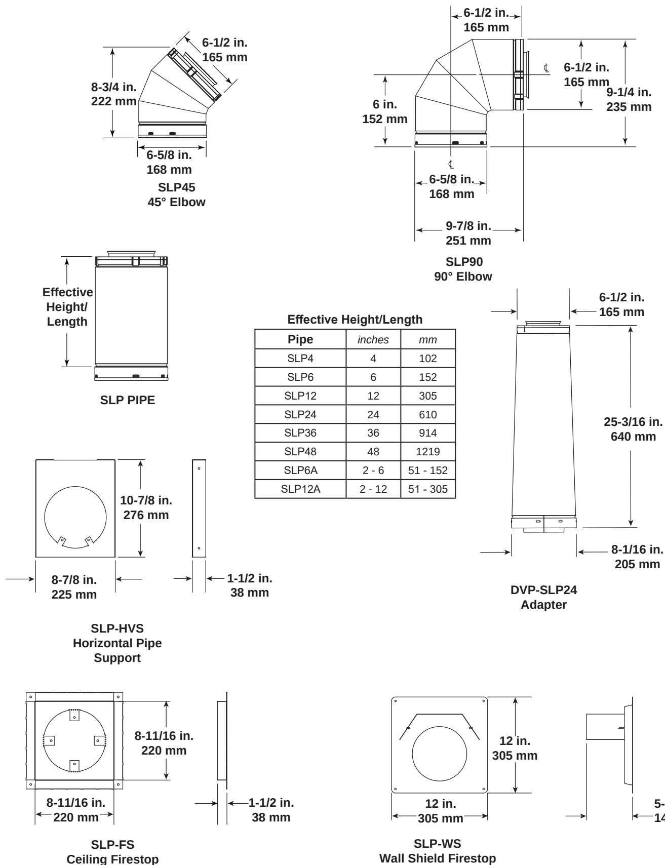
Figure 12.8 SLP Series Vent Components
