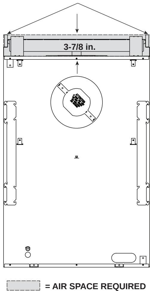
Figure 3.7 Non-Combustible Zone
