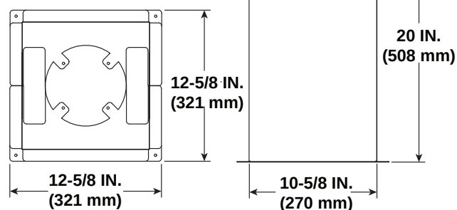
SLP-RDS ROOF DECK INSULATION SHIELD
