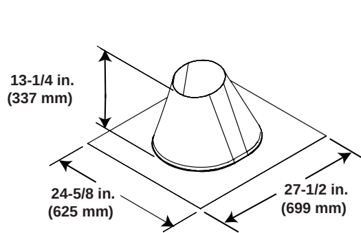
RF6 Roof Flashing
