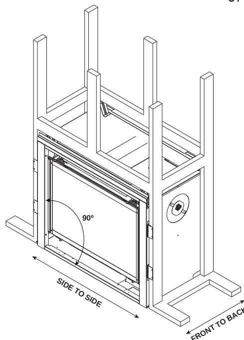
Figure 6.10 Proper Positioning and Leveling of an Appliance
