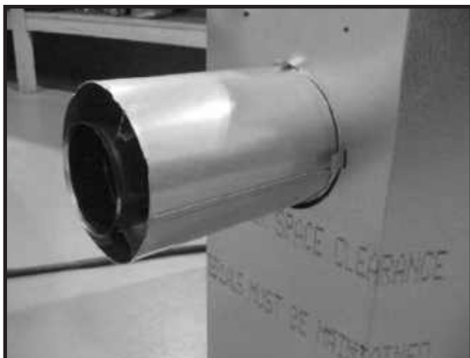
Figure 6.9 Attach the first vent section (it will snap into place). Slide the vent gasket onto the vent section and then, up against the appliance. Secure the vent gasket to the appliance with two self-tapping screws found in the manual bag. Note: The vent gasket can found in the manual bag.
